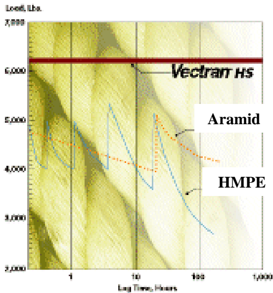
Vectran HS Wire Rope Creep
