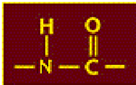
Amide group
