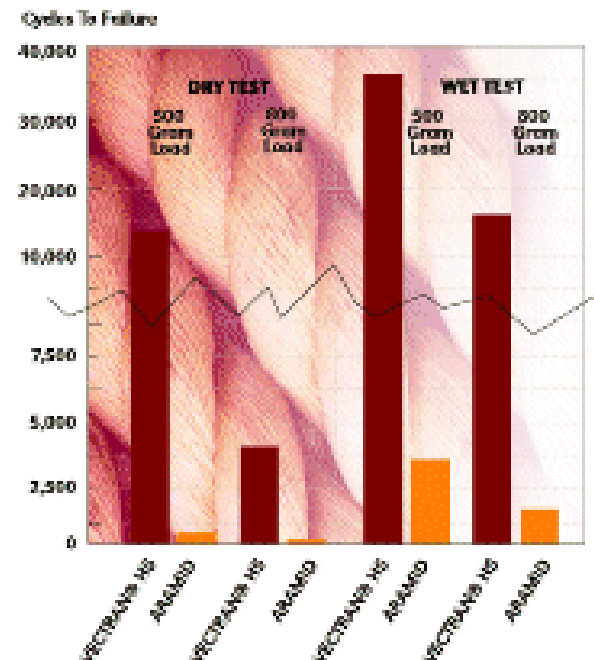
Vectran HS Fiber Abrasion Comparison
